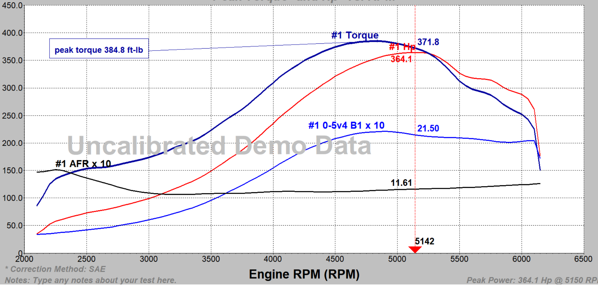
Peak Torque* and Hp* vs. RPM
